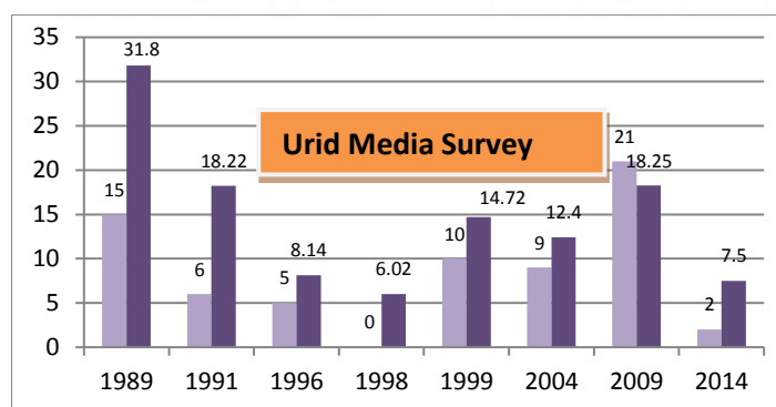
BSP 1989-2014
